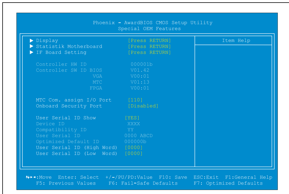
Abbildung 217: Special OEM Features
