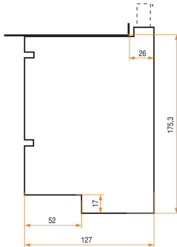
B&R ISA 16 Bit Half Size Karte
