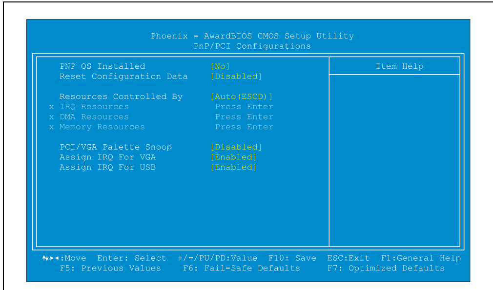
Abbildung 222: PnP/PCI Configurations Setup
