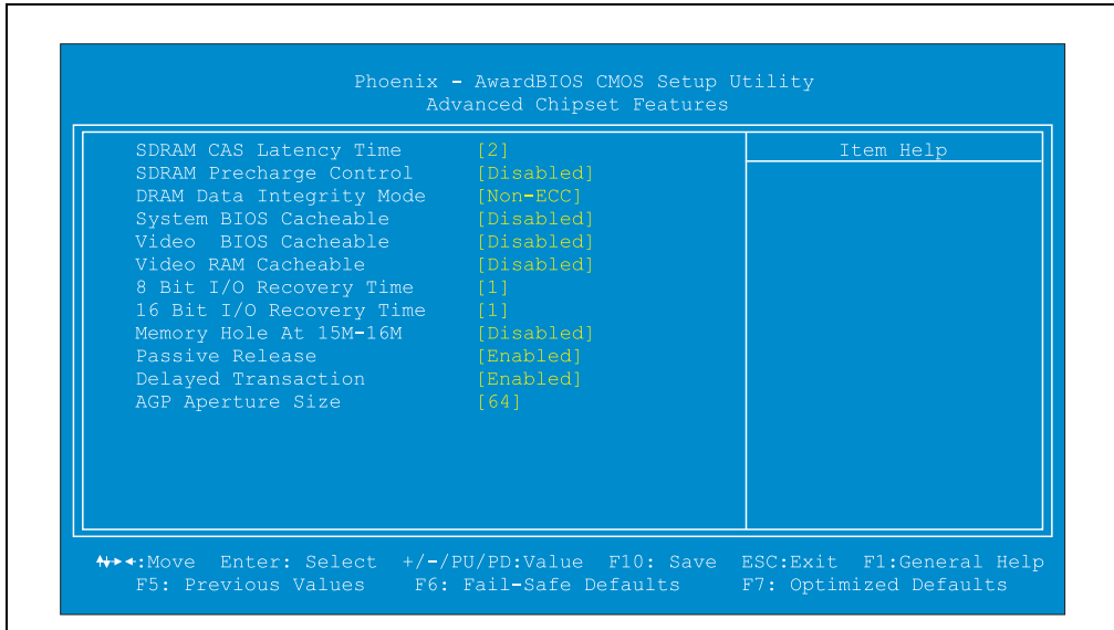
Abbildung 215: Advanced Chipset Features
