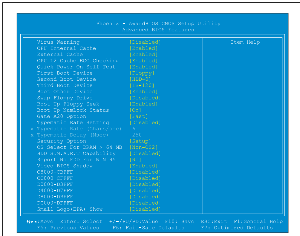
Abbildung 214: Advanced BIOS Features
