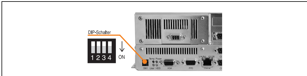
Abbildung 239: IPC5000C/IPC5600C Recovery Jumper
