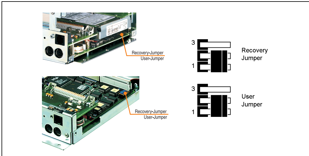
Abbildung 238: IPC5000/IPC5600 Recovery Jumper
