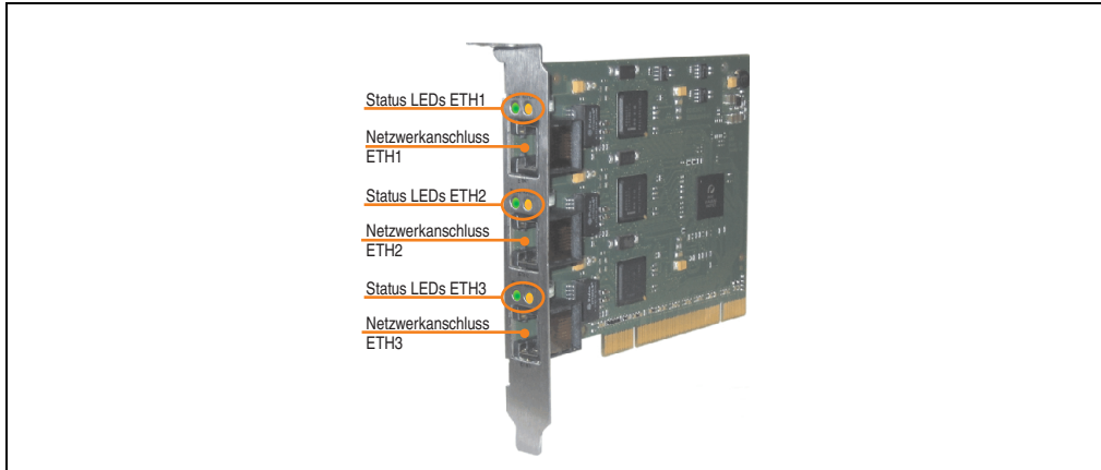
Abbildung 49: PCI Ethernet Card 10/100 - 5ACPCI.ETH3-01
