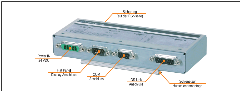
Abbildung 35: Remote Display Adapter - Local Unit 5A5010.01 Anschlüsse
