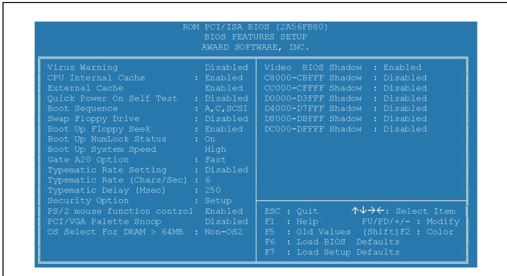
Abbildung 202: BIOS Features Setup
