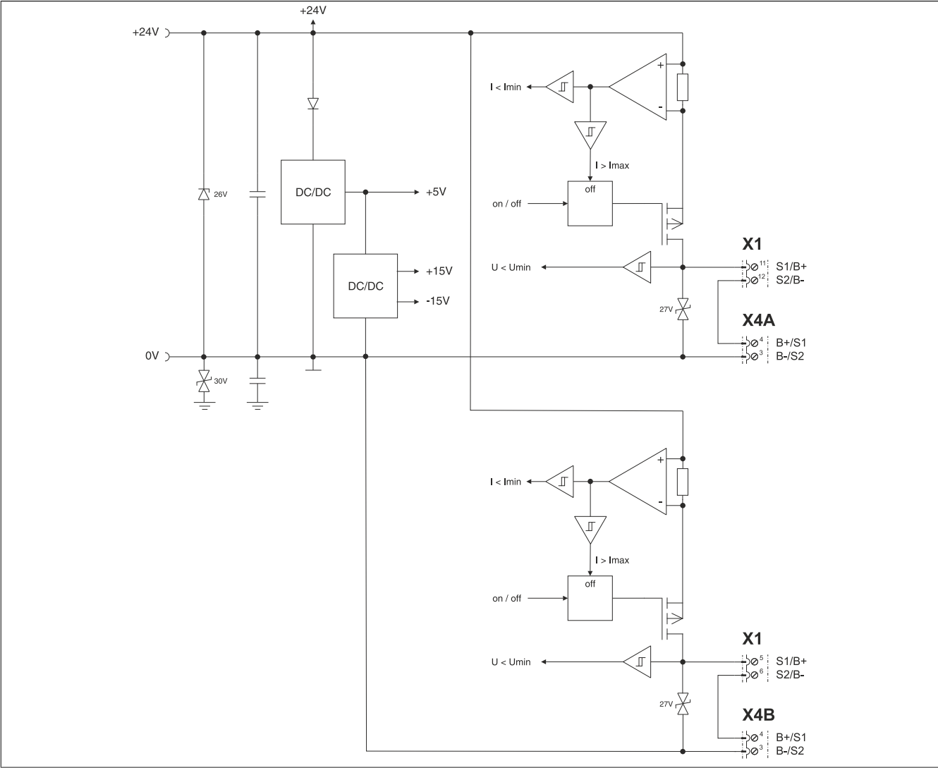
Figure 7: Holding brake
