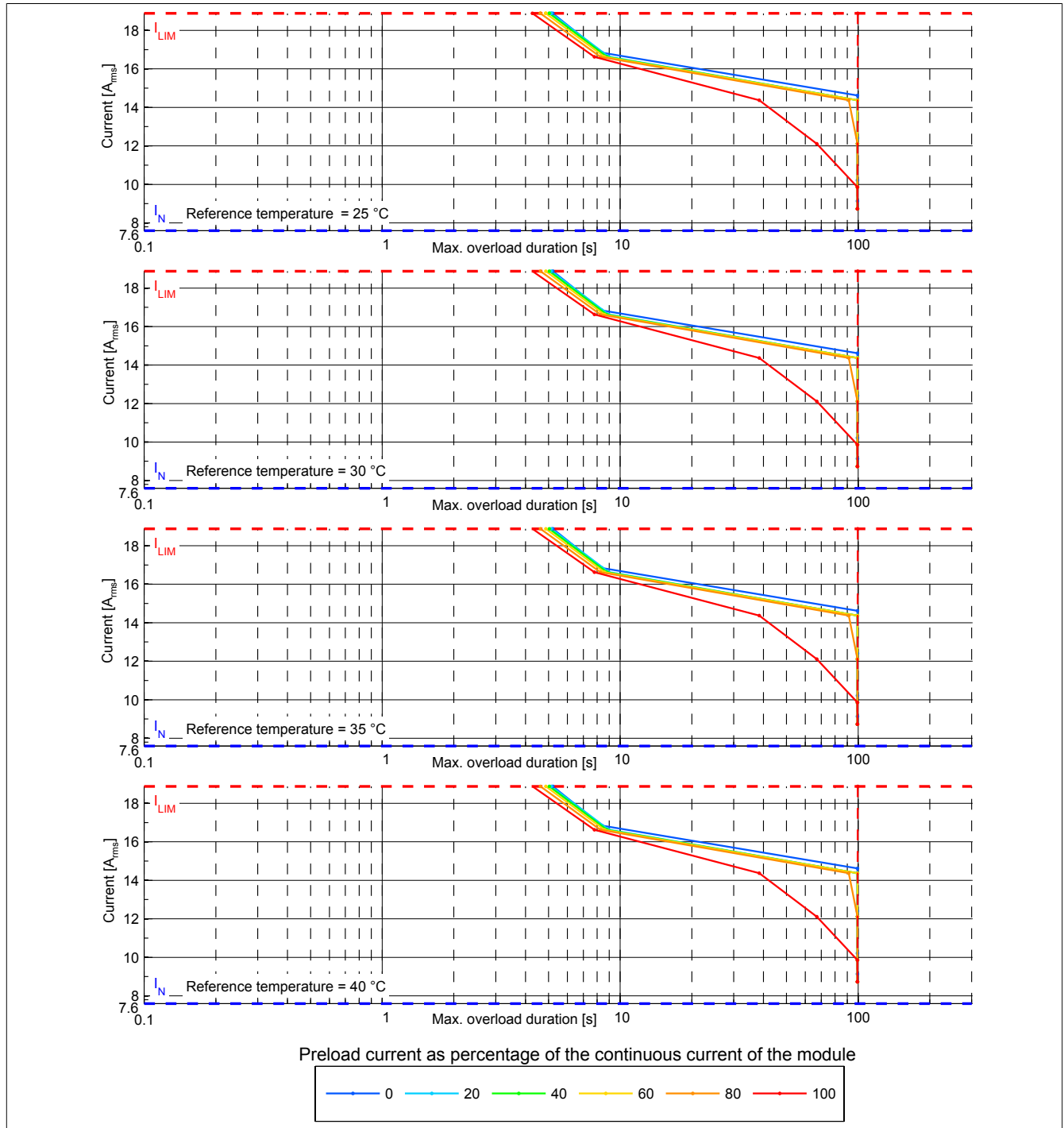
Figure 1: 8BVI0055HWDx.000-1 - Overload characteristics, overload response - WARNING
