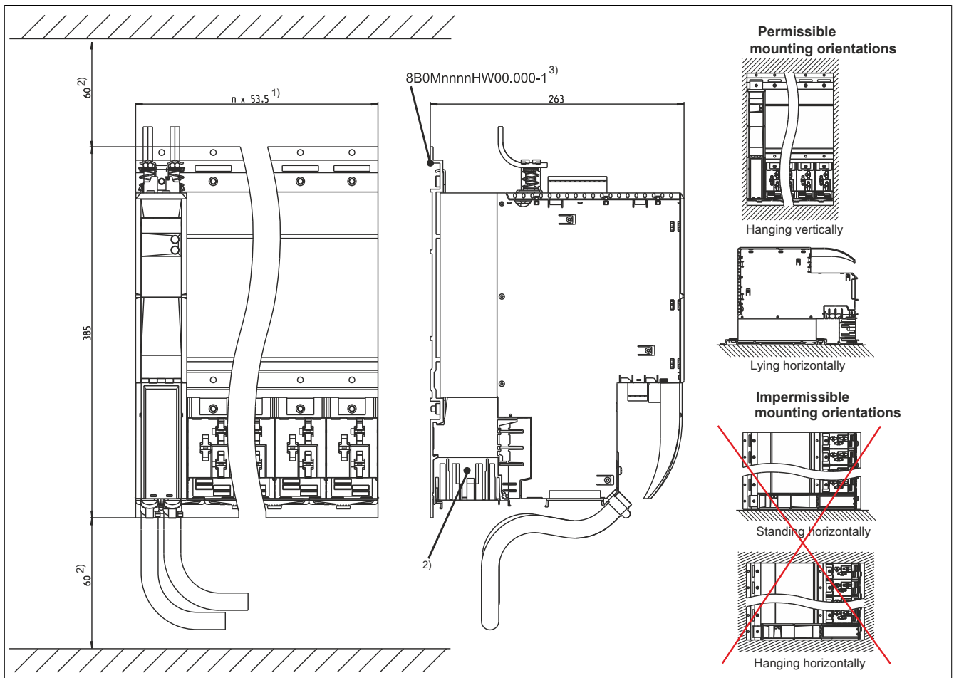
Figure 4: Dimension diagram and installation dimensions
