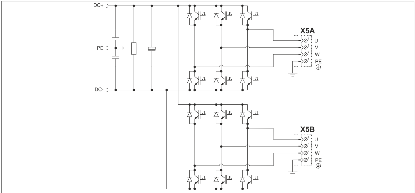
Figure 9: Motor
