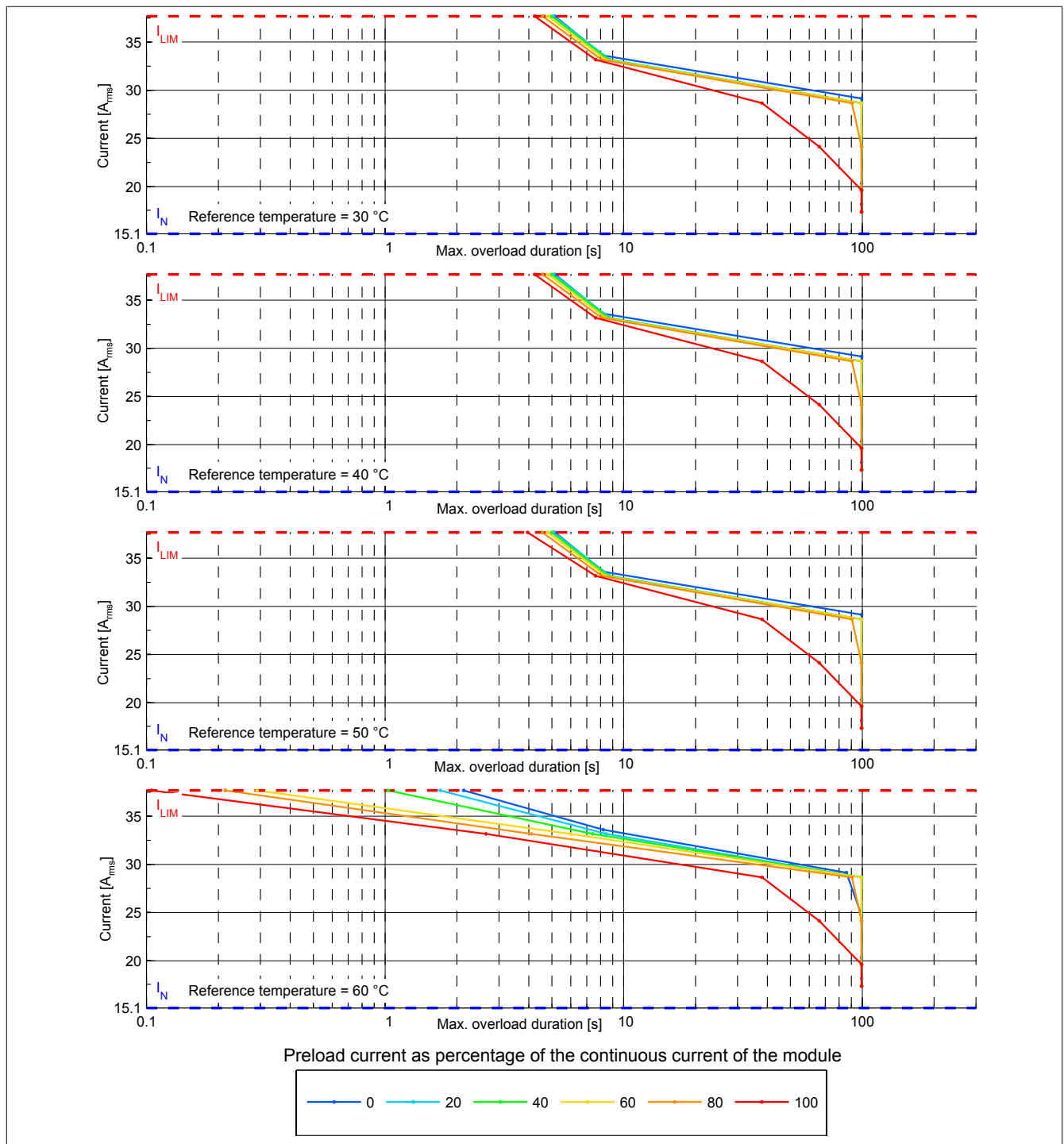
Figure 2: 8BVI0110HCDx.000-1 - Overload characteristics, overload response - ERROR+STOP
