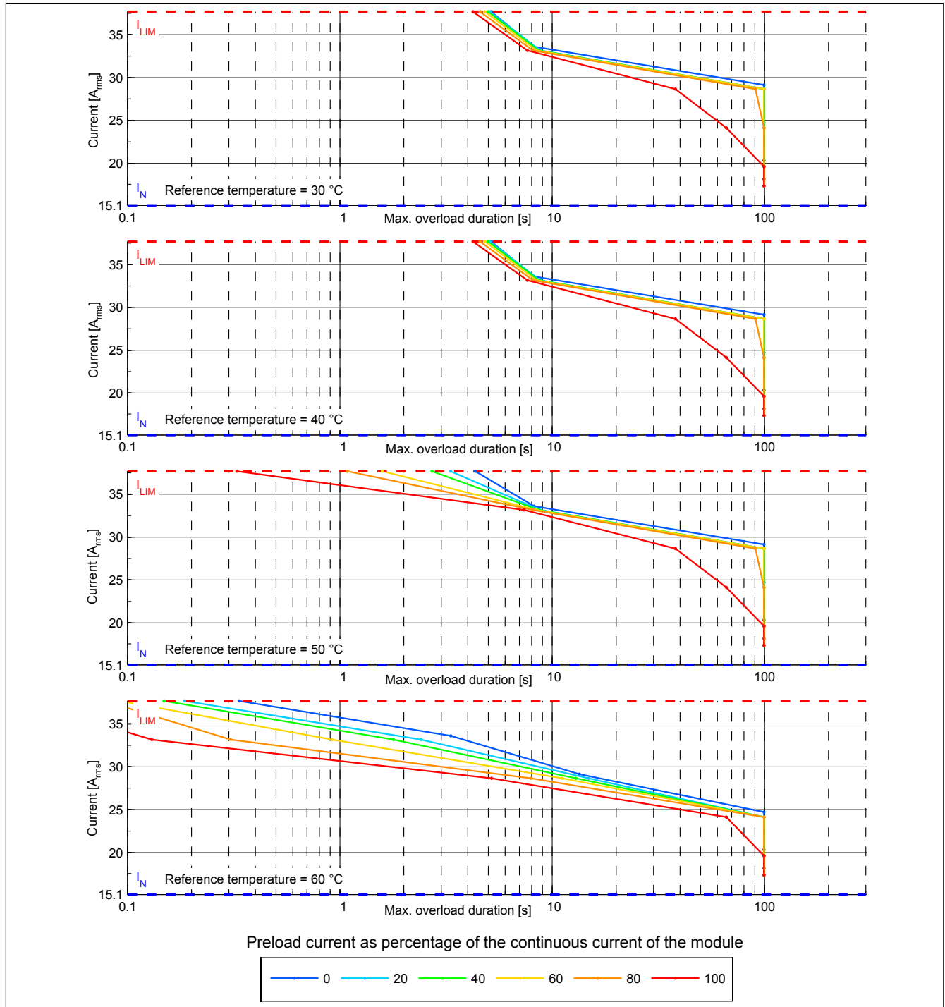
Figure 1: 8BVI0110HCDx.000-1 - Overload characteristics, overload response - WARNING
