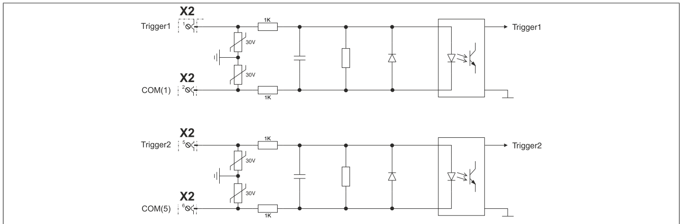
Figure 8: Trigger inputs
