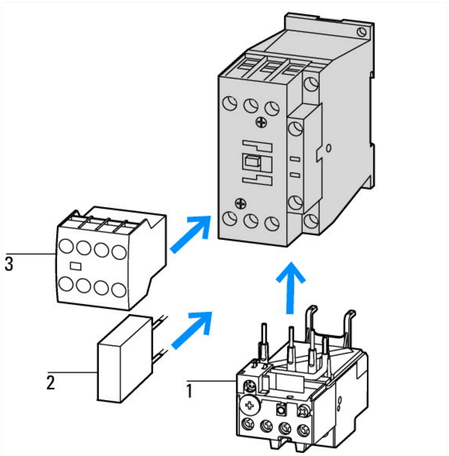
1: Motorschutzrelais
