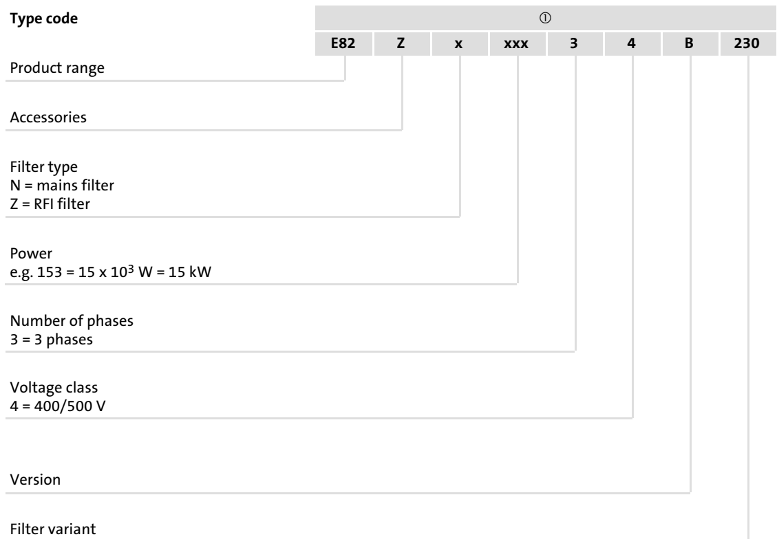
Fig. 3-1 Nameplate
