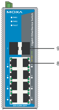
EDS-G308-2SFP Front Panel View
