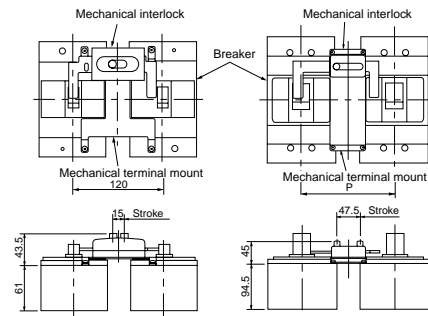
External dimensions
