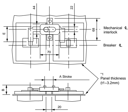
External dimensions
