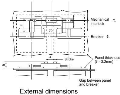
External dimensions
