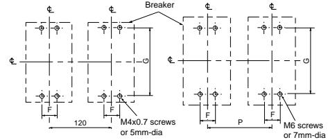
Drilling plan (breaker mount) Fig.2 Fig.3
