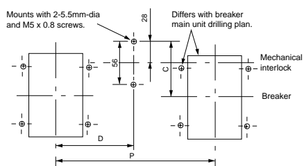
Drilling plan
