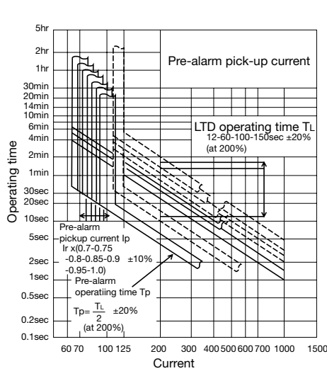
Percentage (%) to rated current or preset current rating (NF/NV100,250AF)
