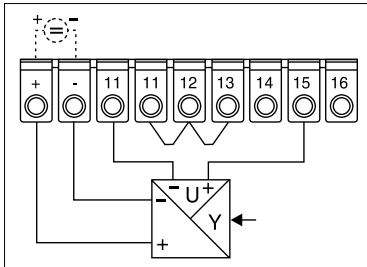
4-wire voltage connection
