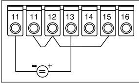
Voltage input \pm 100 mV
