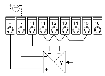
4-wire current connection
