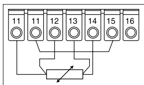
4-wire connection
