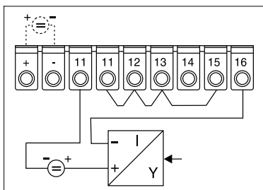
Raccordement courant 2 fils (external powered)
