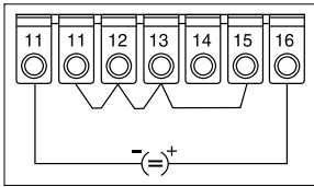
Stroomingang \pm 20\text{mA} , 0/4...20mA
