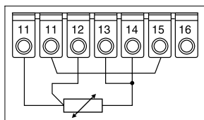
3-wire connection
