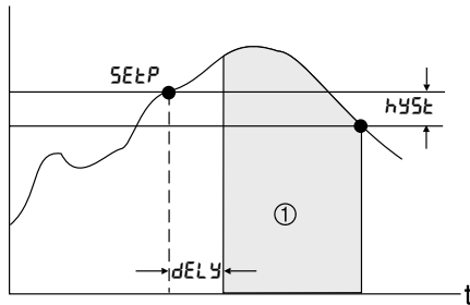
① Relais spanningsloos
