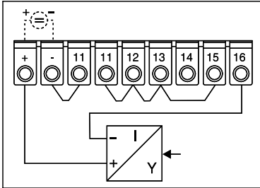
2-wire current connection (loop powered)
