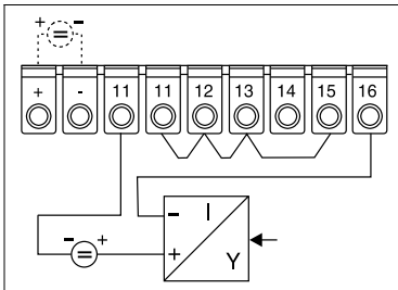
2-Leiter Strom-Anschluss (External powered)
