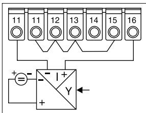
4-wire current connection
