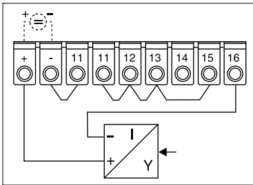
2-Leiter Strom-Anschluss (Loop powered)
