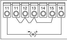
Current input \pm 20 mA, 0/4 to 20 mA
