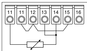
2-wire connection
