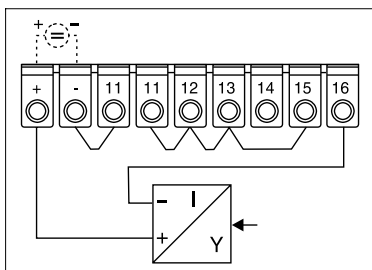
Raccordement courant 2 fils (Loop powered)
