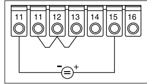
Voltage input \pm 10 V, 0 to 1/10 V
