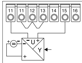
4-wire voltage connection
