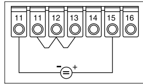
Spanningsingang \pm 10\text{V} , 0...1/10V
