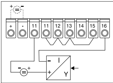
2-wire current connection (external powered)
