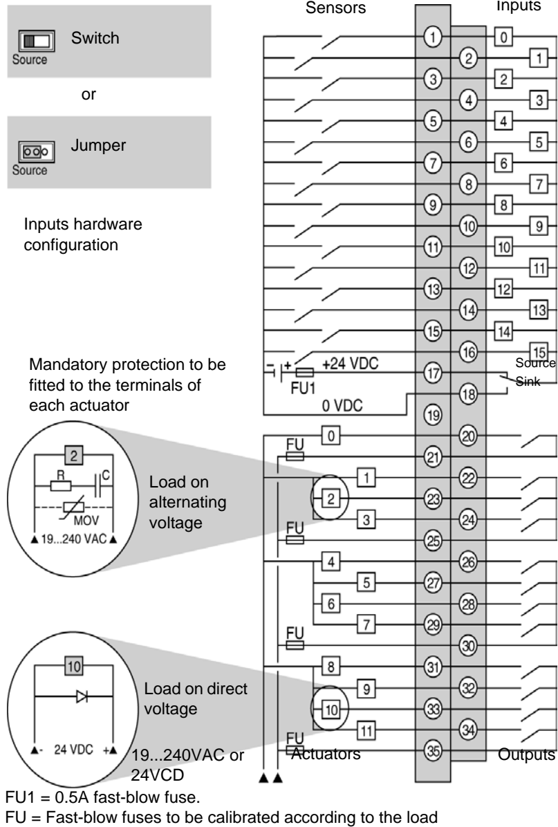
Diagram of TSX DMZ 28DR ("Source" negative logic inputs)
